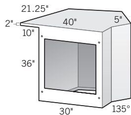
135° Corner Cabinet with 10" Cantilever 30"D × 36"H • OLPLSCC45
