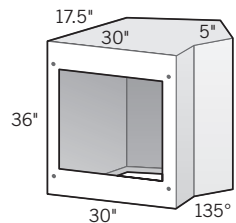
135° Corner Cabinet 30"D × 36"H • OLPLSCH45
