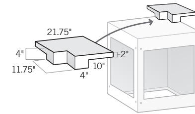
Corner Raised Backsplash OLPLSBCRN Creates 4" high raised corner backsplash with 10" cantilever; connects to Straight Raised Backsplash for L-shaped configurations. Requires 2 bolts for mounting (not included).
