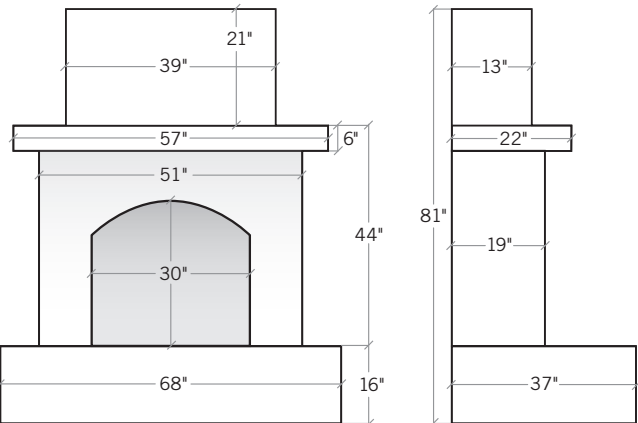
Gas-Burning Fireplace 37" D x 68" L x 81" H • OLPLSFP01
