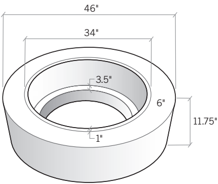
Fire Pit 46" DIAMETER x 11.75" H • OLPLSFP48
