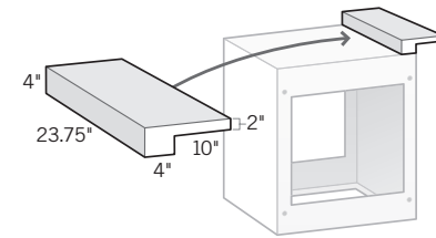
Straight Raised Backsplash OLPLSBSTR Creates 4" high raised backsplash (23.75" long) with 10" cantilever and 14" counter surface. Requires 3 bolts for mounting (not included).
