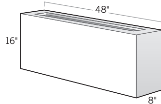
Straight Seating Wall 8"D × 48"L × 16"H • OLPW81648 Create seating walls in hours vs. days. Finish with Eldorado Stone & Wall Caps for an authentic masonry appearance.
