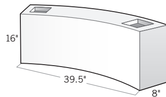
Curved Seating Wall (1/8 Circle) 8"D × 39.5"L × 16"H • OLPW81640 Curved seating wall is designed with a 51" radius from the center point to the inside edge, perfect for pairing with our round fire pit.
